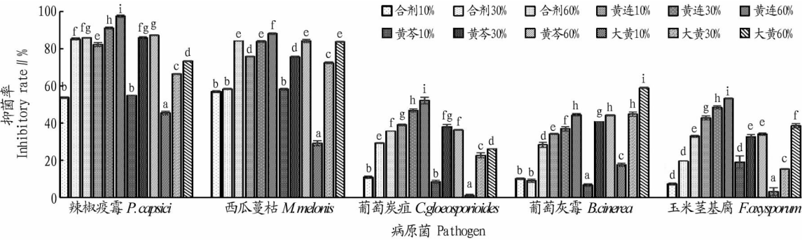
图 1 不同浓度的水浸提液复合剂对菌株的抑菌效果 Fig. 1 Inhibitory effect of different extracts with different concentrations on growth of five pathogens
